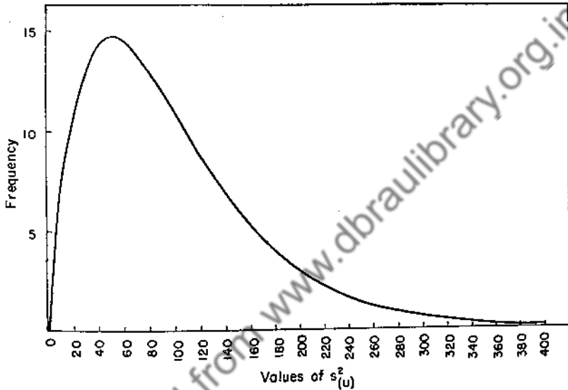
Figure 2. The Chi-square distribution curve based on the unbiased estimates of the variance, s^2(u) 's, of 100 random samples of 5 from a normal population with mean 30 and variance 100 (Table 10).
